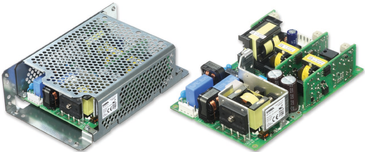
Figure 01 –COSEL RBC200F triple isolated outputs for small and medium robotic and factory automation
