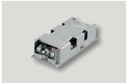
Defense line 300 DC 300W, Enclosed, rugged design DC/DC converter 12, 24, 48, 72, 110VDC inputs Output from 3V3 to 48VDC
